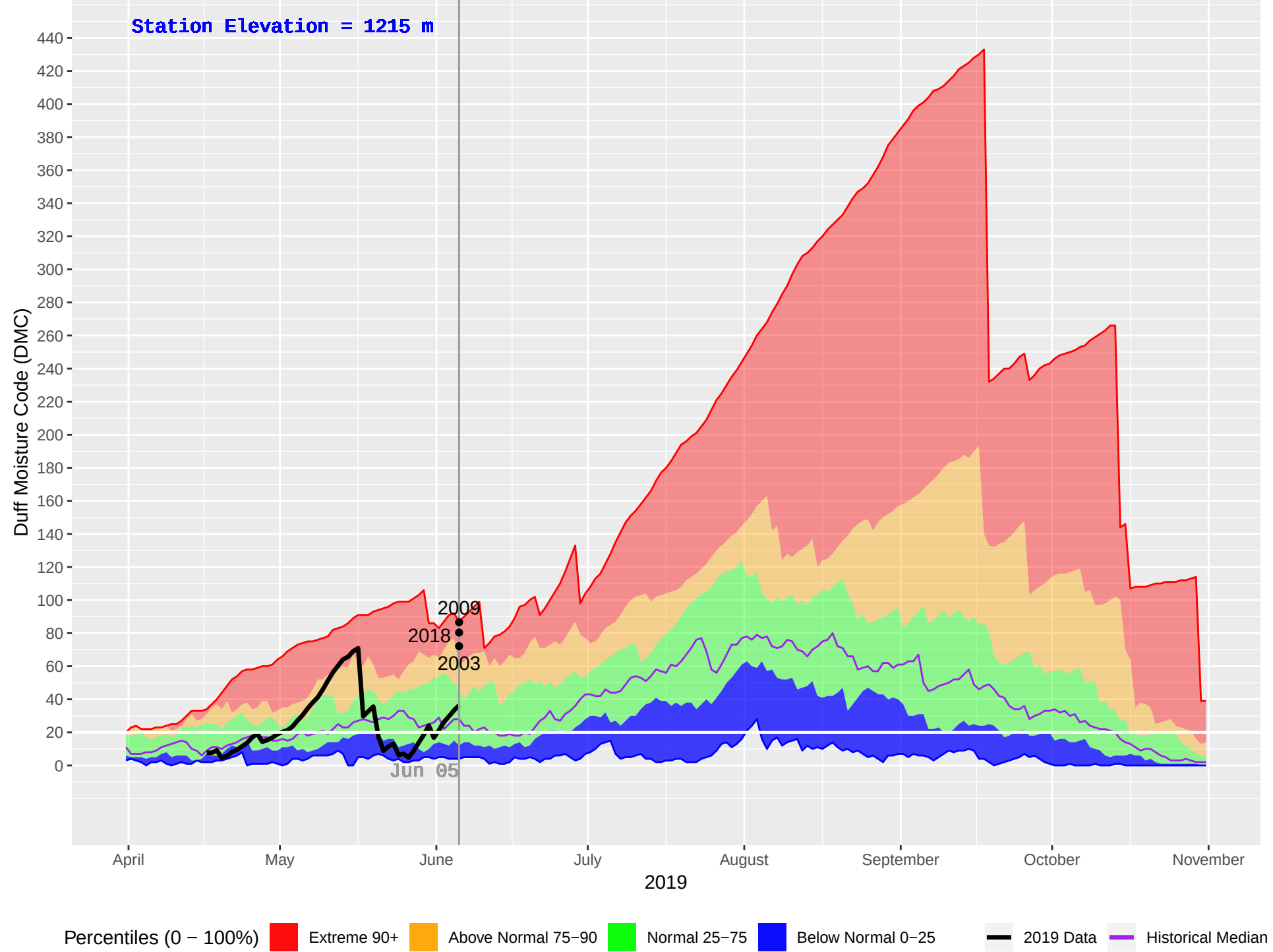
ALLISON PASS (317) : Historical (1987–2018), Current (2019) Daily Duff Moisture Code (DMC)
