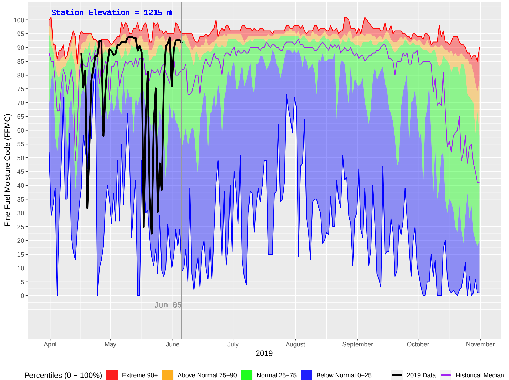
ALLISON PASS (317) : Historical (1987–2018) and Current (2019) Daily Fine Fuel Moisture Code (FFMC)
