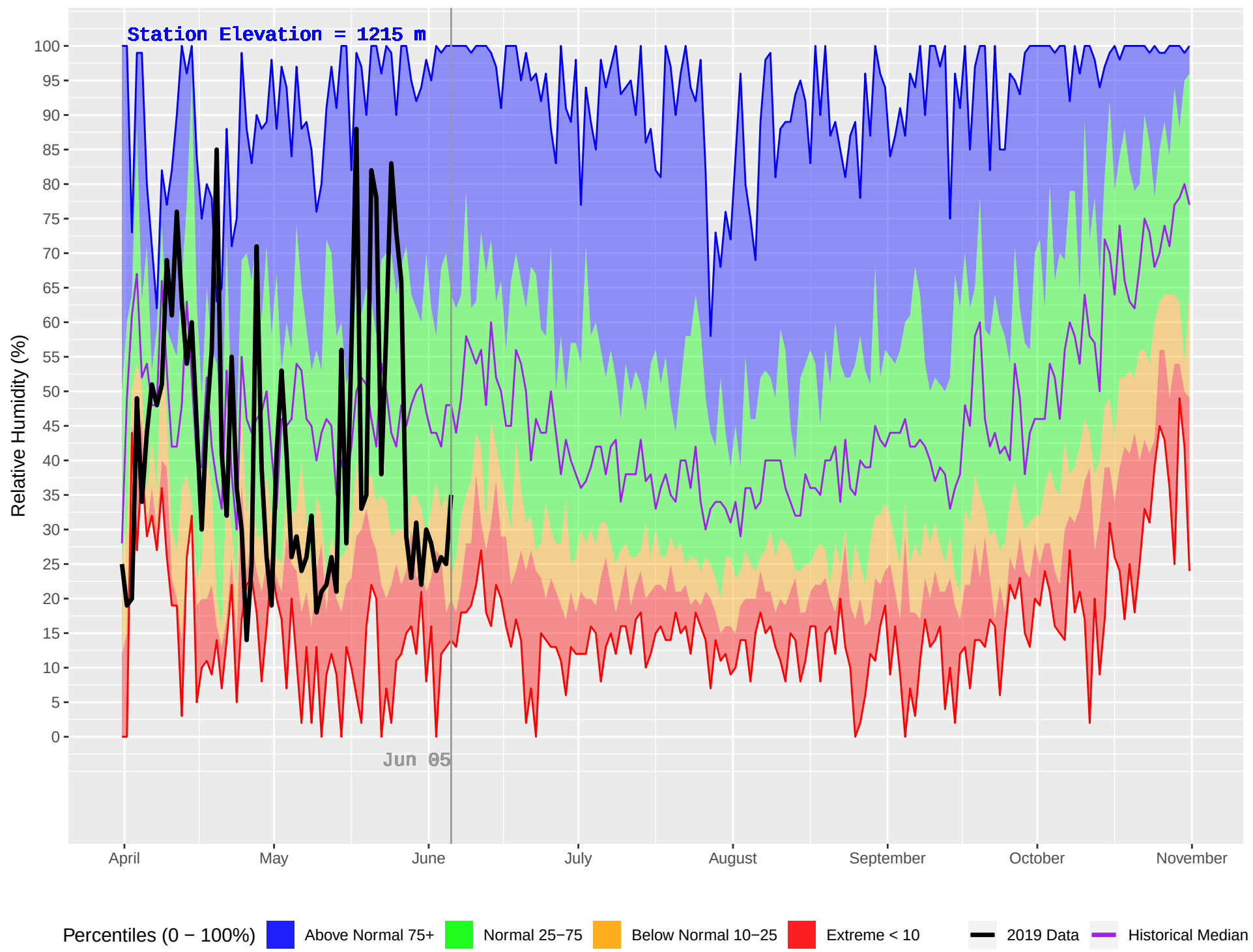
ALLISON PASS (317) : Historical (1987–2018) and Current (2019) Daily Relative Humidity
