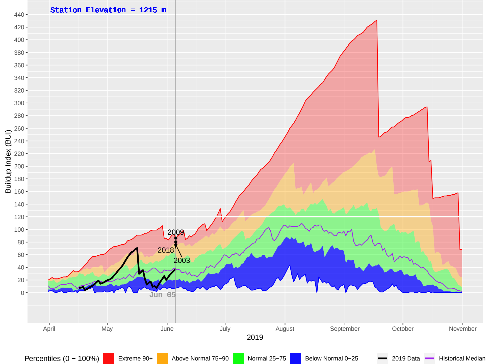
ALLISON PASS (317) : Historical (1987–2018), Current (2019) Daily Buildup Index (BUI)
