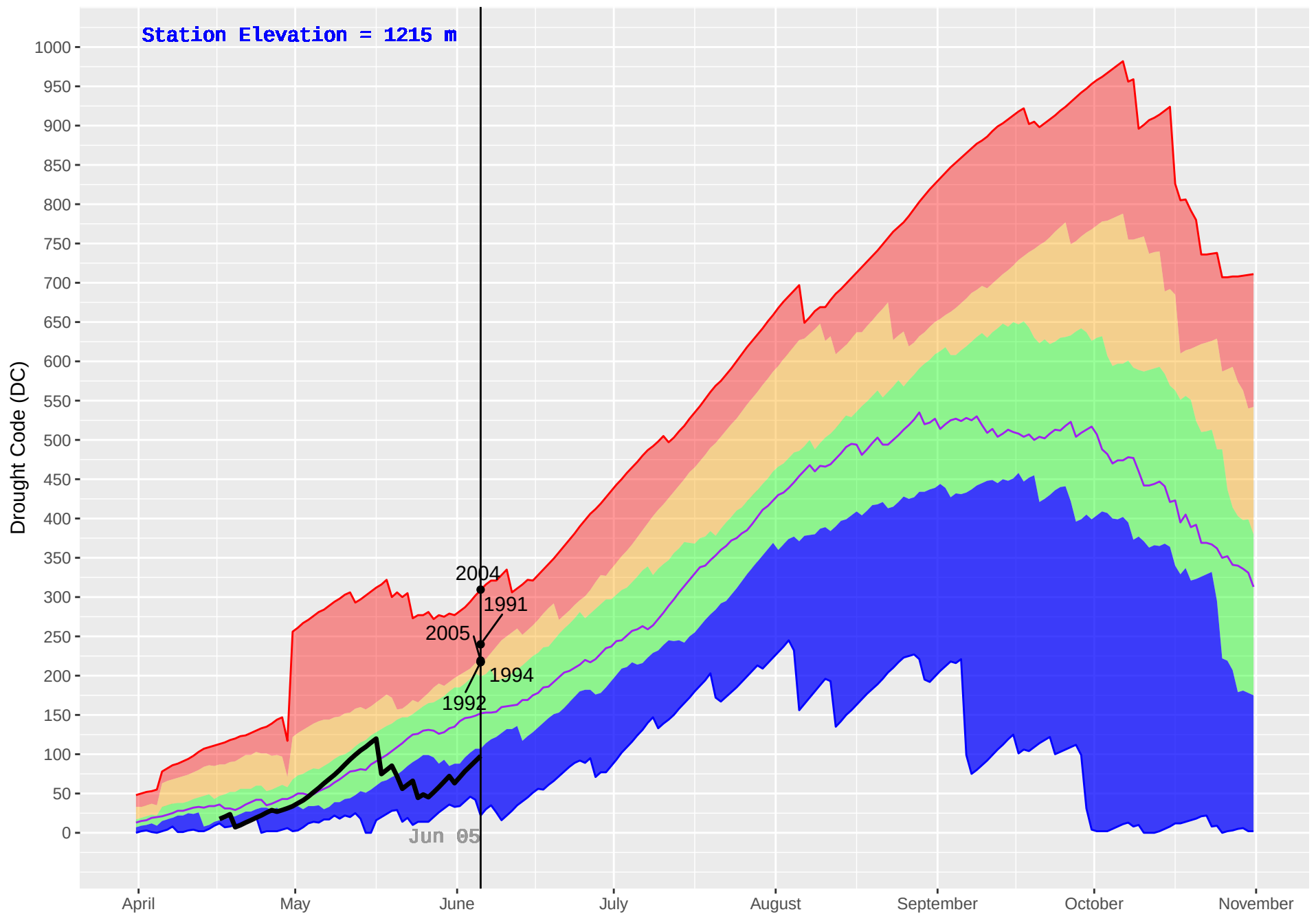
ALLISON PASS (317) : Historical (1987–2018) and Current (2019) Daily Drought Code (DC)
